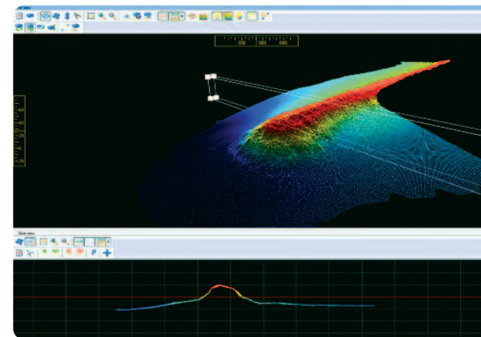
Combined Point Cloud from Dynascan and Sonar of Breakwater
